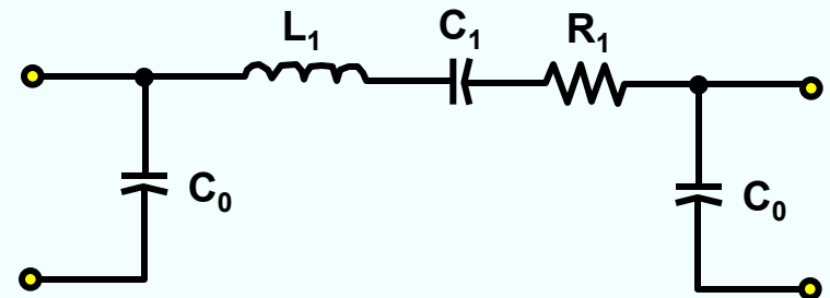
Two-port SAW
