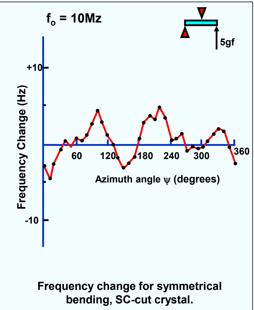
SC-cut resonator
