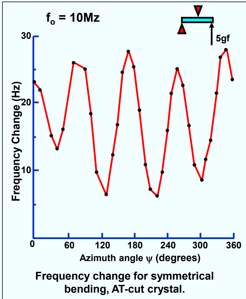
AT-cut resonator
