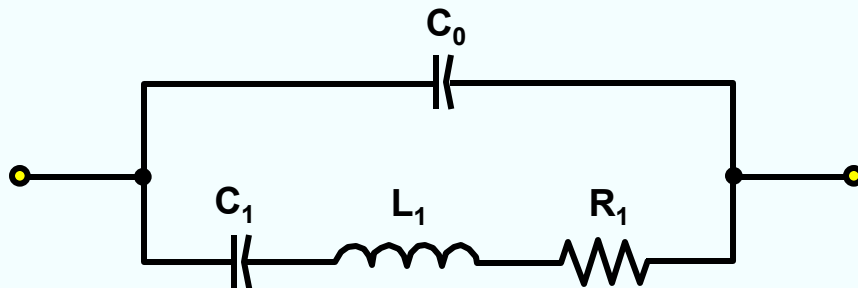
BAW and One-port SAW
